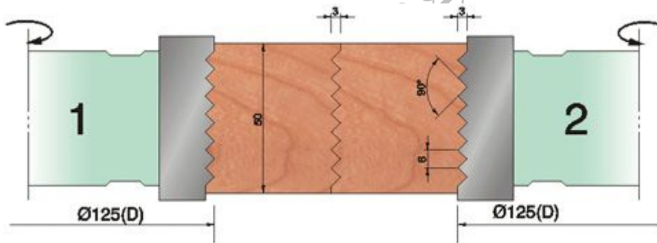
TF619B D125*d40*Z4 1SET/2PCS
